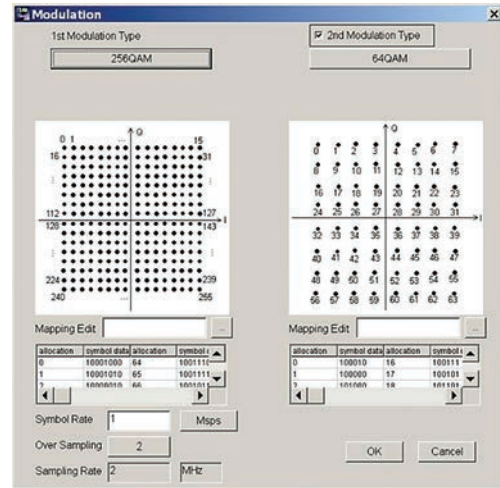
Modulation Screen
