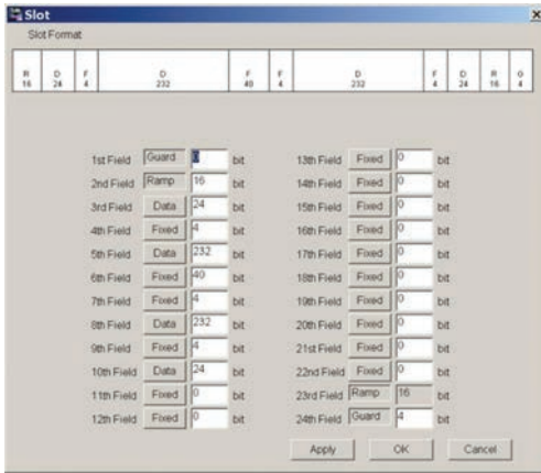
Slot Screen
